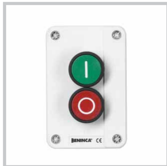
IPB.NC Industrial keypad fitted with a contact that is normally open and a contact normally closed
